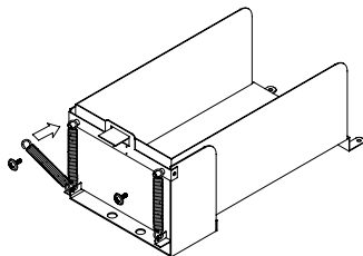
Figure 35 – Spring Replacement
