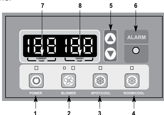
Figure 32 – Control Panel
